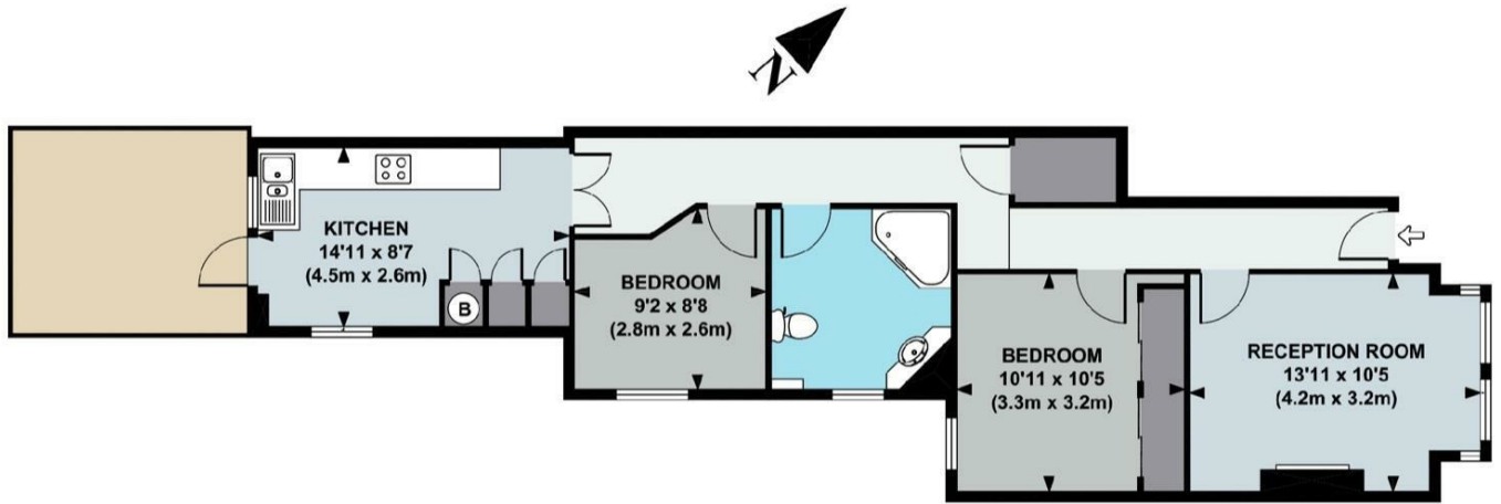
FIRST FLOOR
