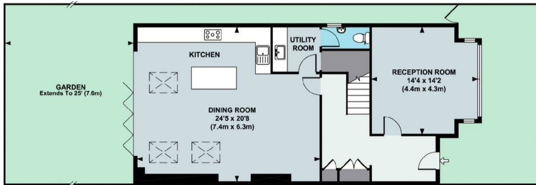
GROUND FLOOR
